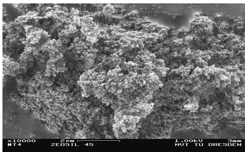
Figure 9: Scanning electron microscope image of precipitated SAS agglomerate
