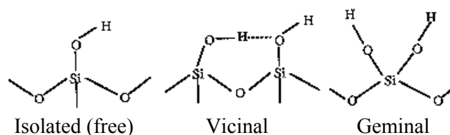
Figure 3: Surface silanol groups on SAS
