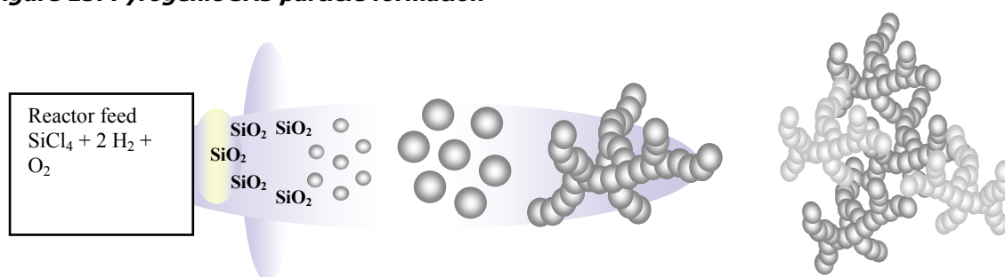
Figure 15: Pyrogenic SAS particle formation
