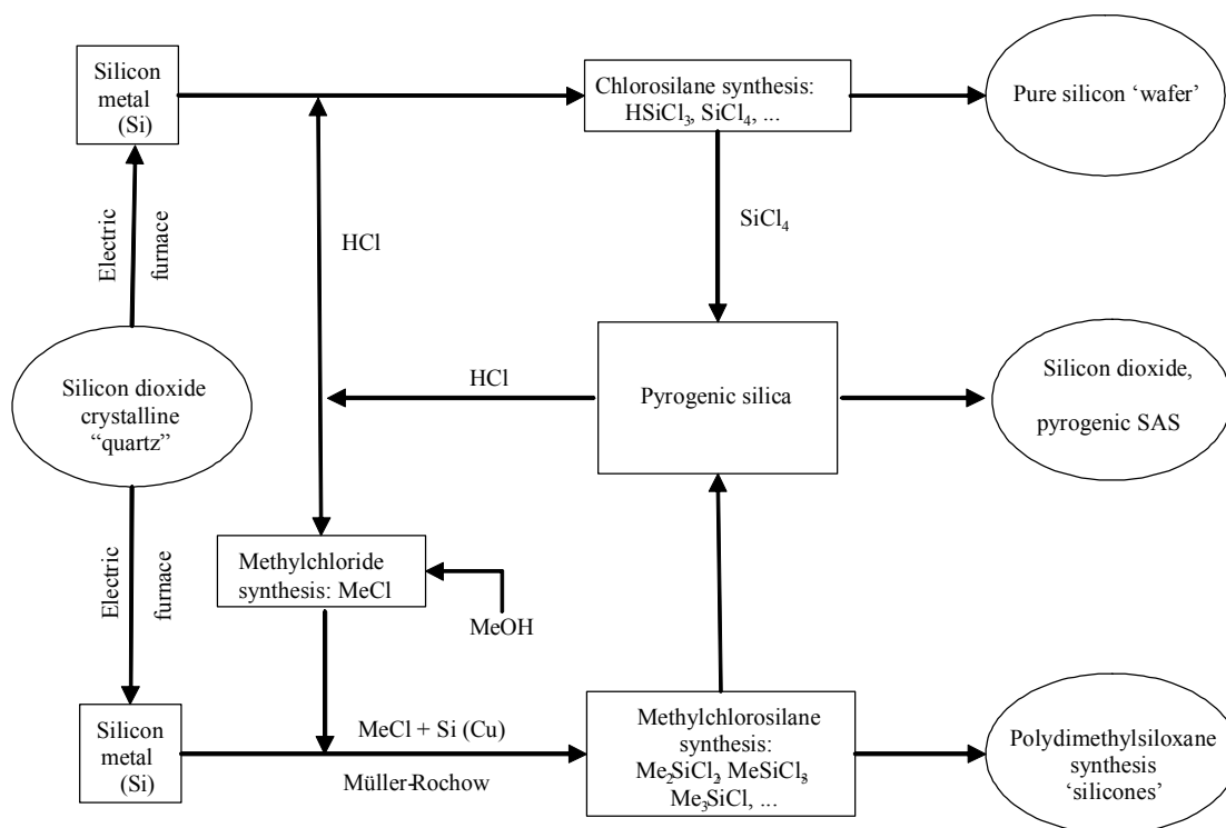
Figure 16: Process flow diagram for the synthesis of pyrogenic SAS
