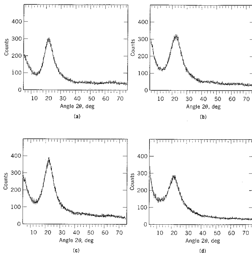
Figure 2: X-ray diffraction pattern of different SASs (Kirk-Othmer, 1997)
