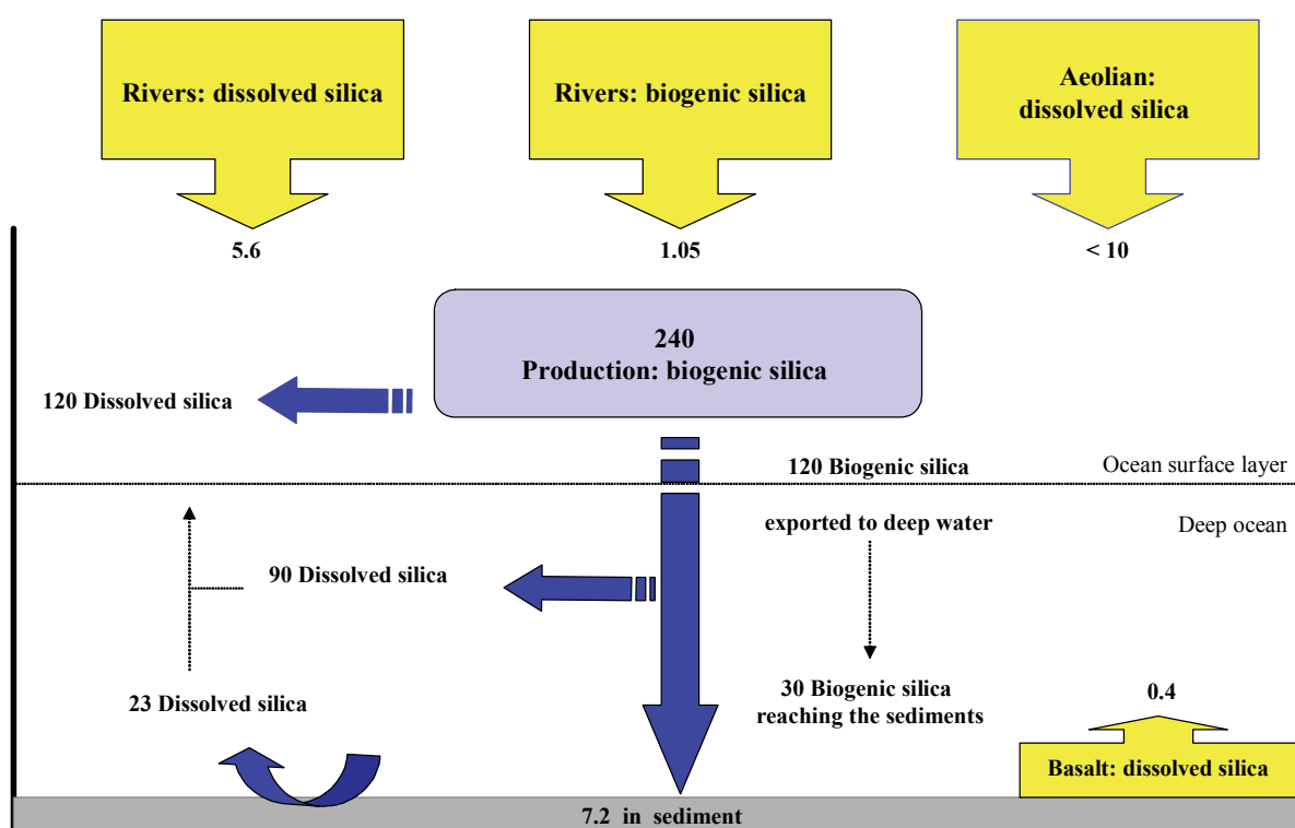
Figure 22: Global biogeochemical silicon cycle a (Nelson et al , 1995; Tréguer et al , 1995)
