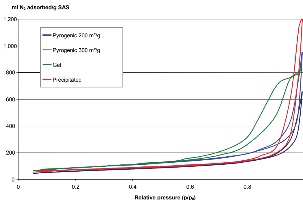
Figure 11: Nitrogen adsorption and desorption isotherms a of different SASs
