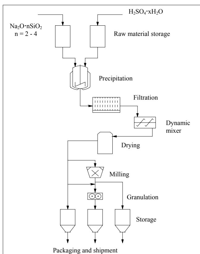
Figure 17: Production of precipitated SAS
