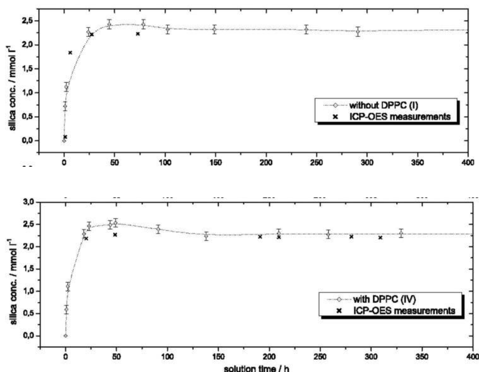
Figure 6: Dissolution of SAS (Cab-O-Sil M5) without and with DPPC a (Roelofs, 2002)
