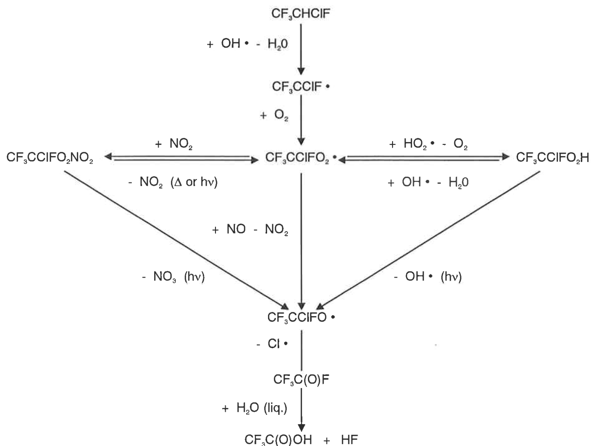
Figure 1 Tropospheric Degradation Mechanism for HCFC-124
