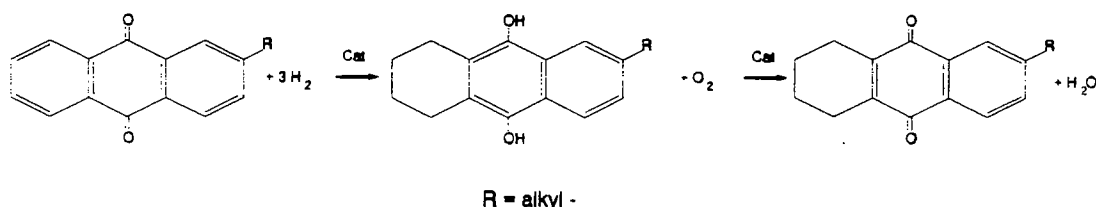
FIGURE 1 ANTHRAQUINONE AUTOXIDATION METHOD (Goor et al , 1989)
