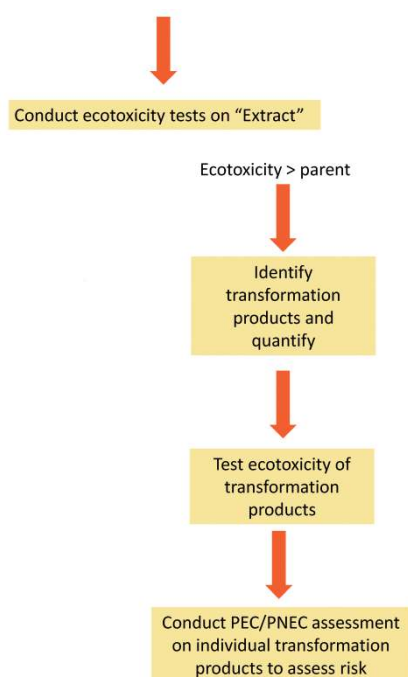
Figure 18: Exposure driven assessment
