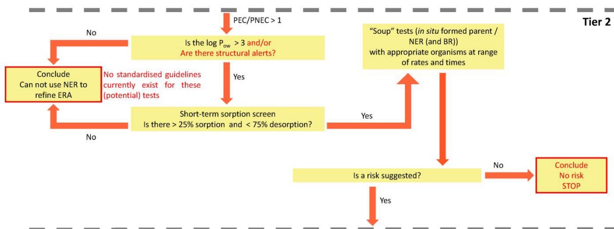
Figure 13: Introduction to the Tier 2 of the NER risk assessment framework
