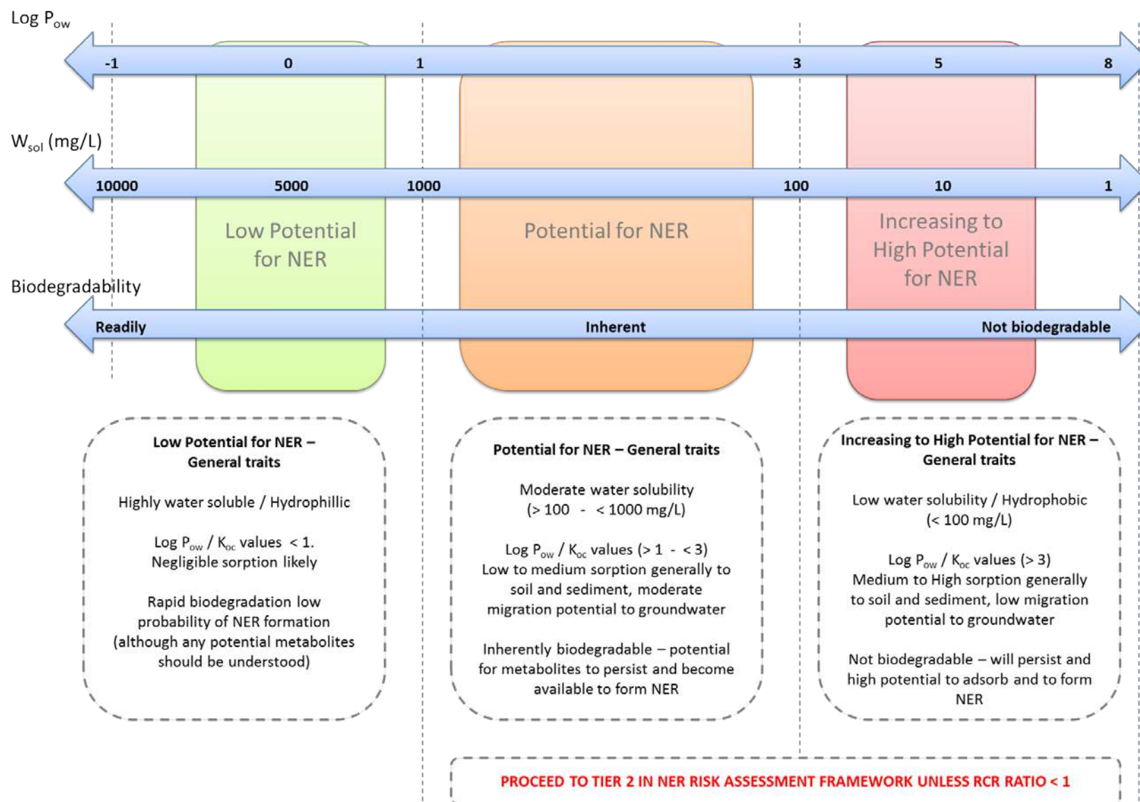
Figure 12: Summary of physico-chemical properties and fate profiles and the subsequent potential for NER formation
