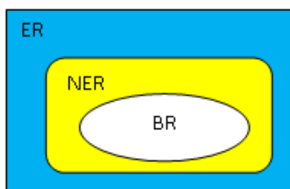
Figure 2: Representation of ER, NER and BR (based on Zarfl et al, 2009)
