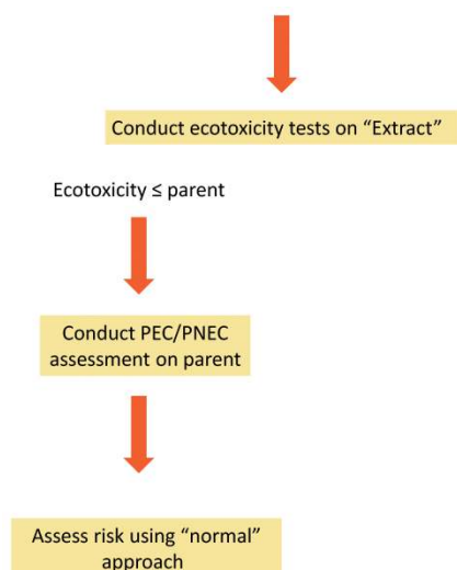
Figure 19: Effects driven assessment
