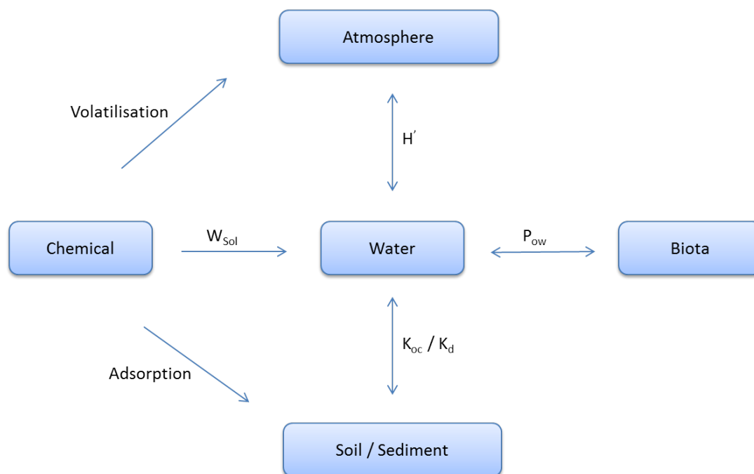
Figure 5: Physico-chemical properties and influence on the compartment in which a chemical will reside
