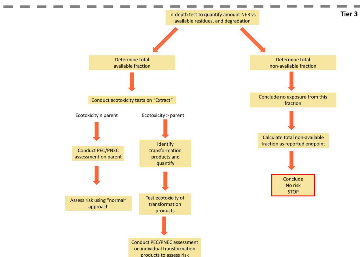
Figure 17: Introduction to Tier 3 of the NER risk assessment framework
