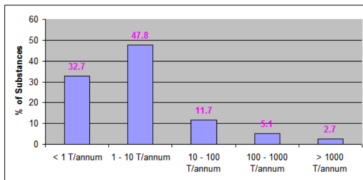
Figure 4: Distribution of substances registered in the EU with respect to their tonnage band (JRC, 2013)
