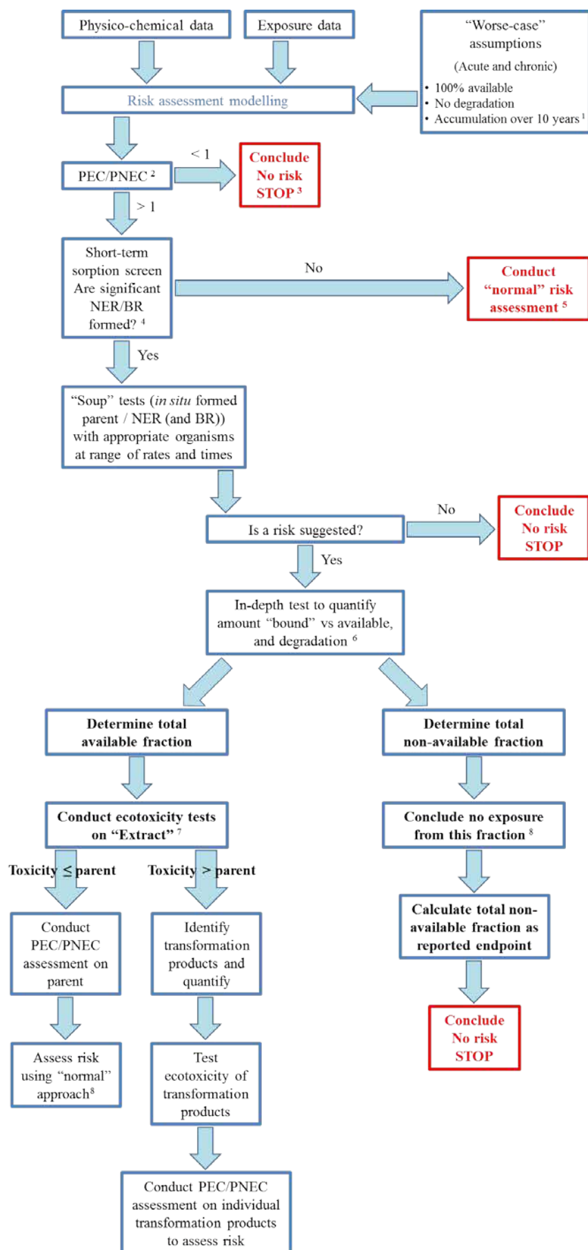
Figure 1: Risk assessment framework accounting for non-extractable residues as proposed by ECETOC (2010)
