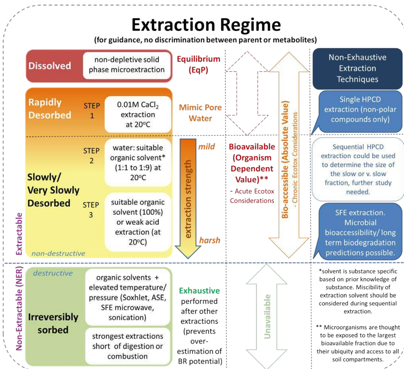
Figure 3: Extraction methodology framework (ECETOC, 2012)
