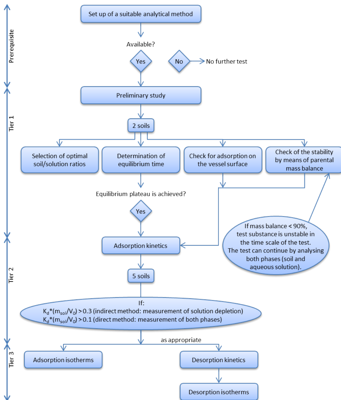
Figure 6: OECD testing scheme, OECD 106 (OECD, 2000a)
