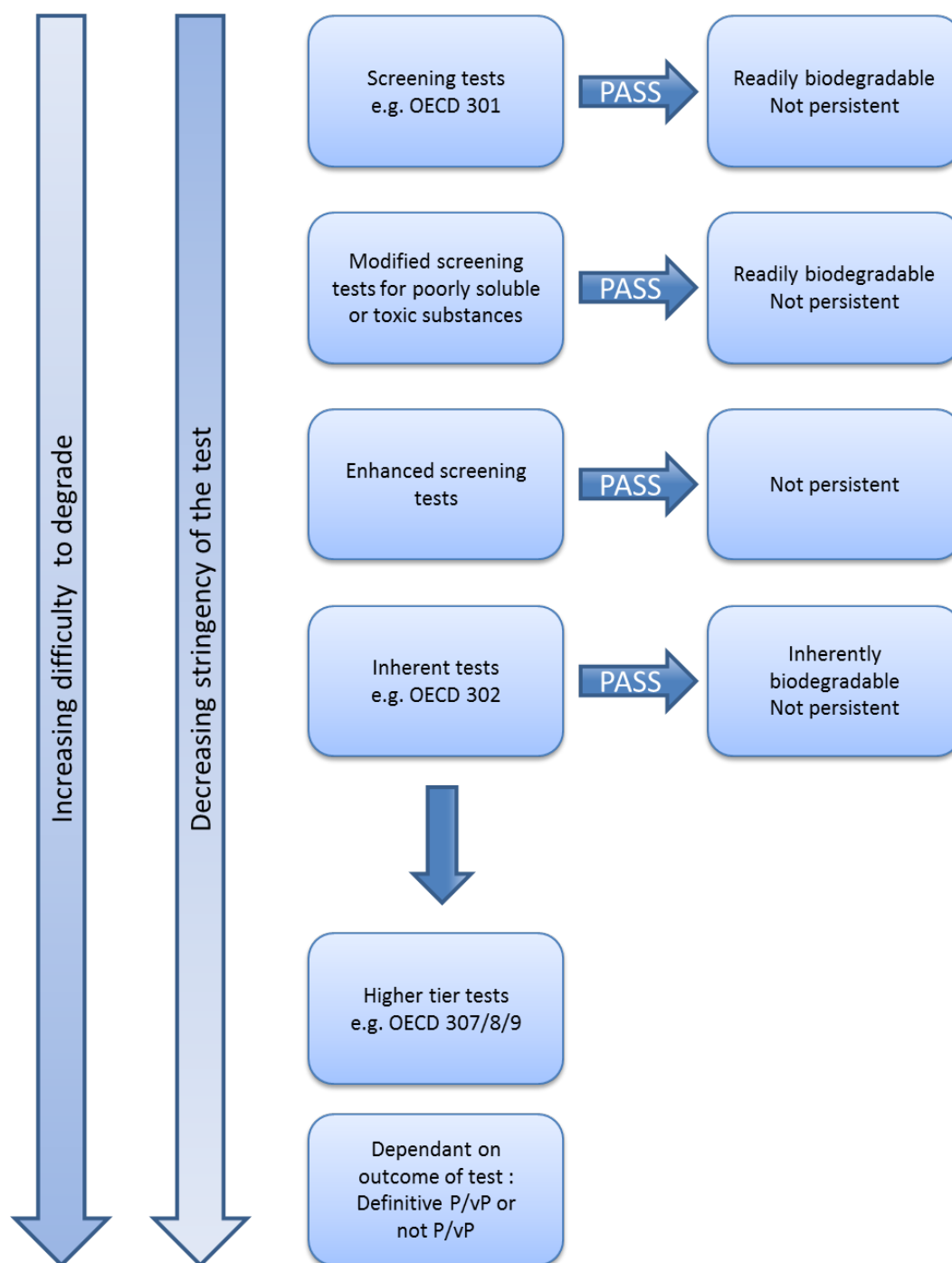
Figure 7: Hierarchy of screening and higher tier biodegradation tests for determining persistence (Comber and Holt, 2010)
