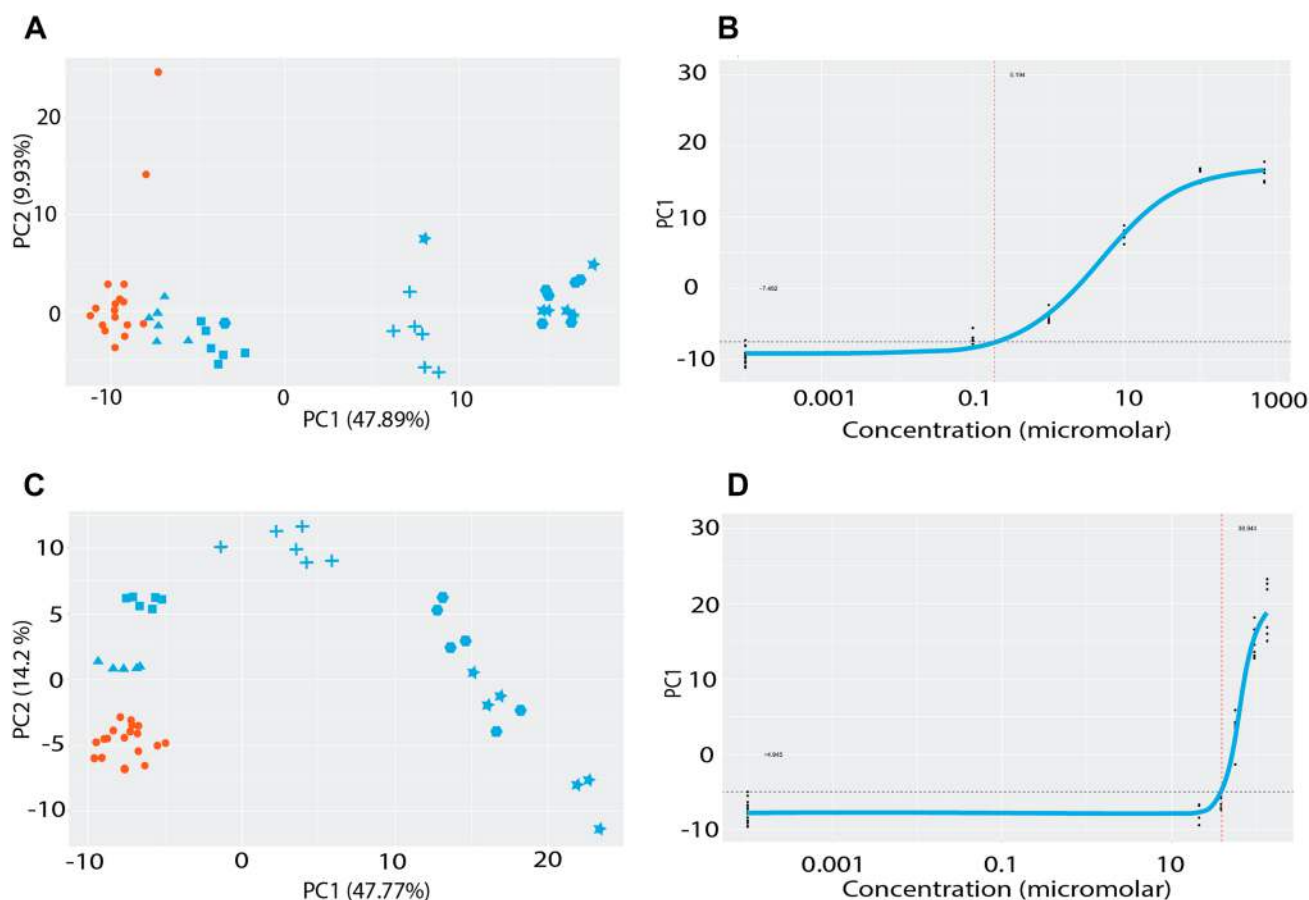
Fig. 4 Examples of deriving PODs using principal component 1 for dose response modelling as described above for \beta - naphthoflavone (A and B) and aroclor (C and D). The PCA plots are shown in A and C
