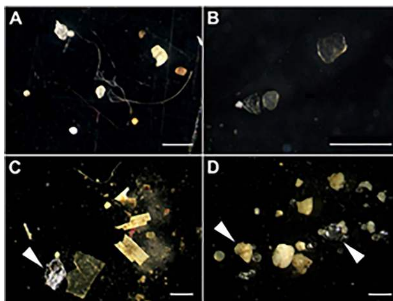
Microplastics in sediment from rivers. By Martin Wagner et al. - Wagner et al.: Microplastics in freshwater ecosystems: what we know and what we need to know. In: Environmental Sciences Europe. 26, 2014, doi:10.1186/s12302-014-0012-7, CC BY 4.0, https://commons.wikimedia.org/w/index.php?curid=3950778
