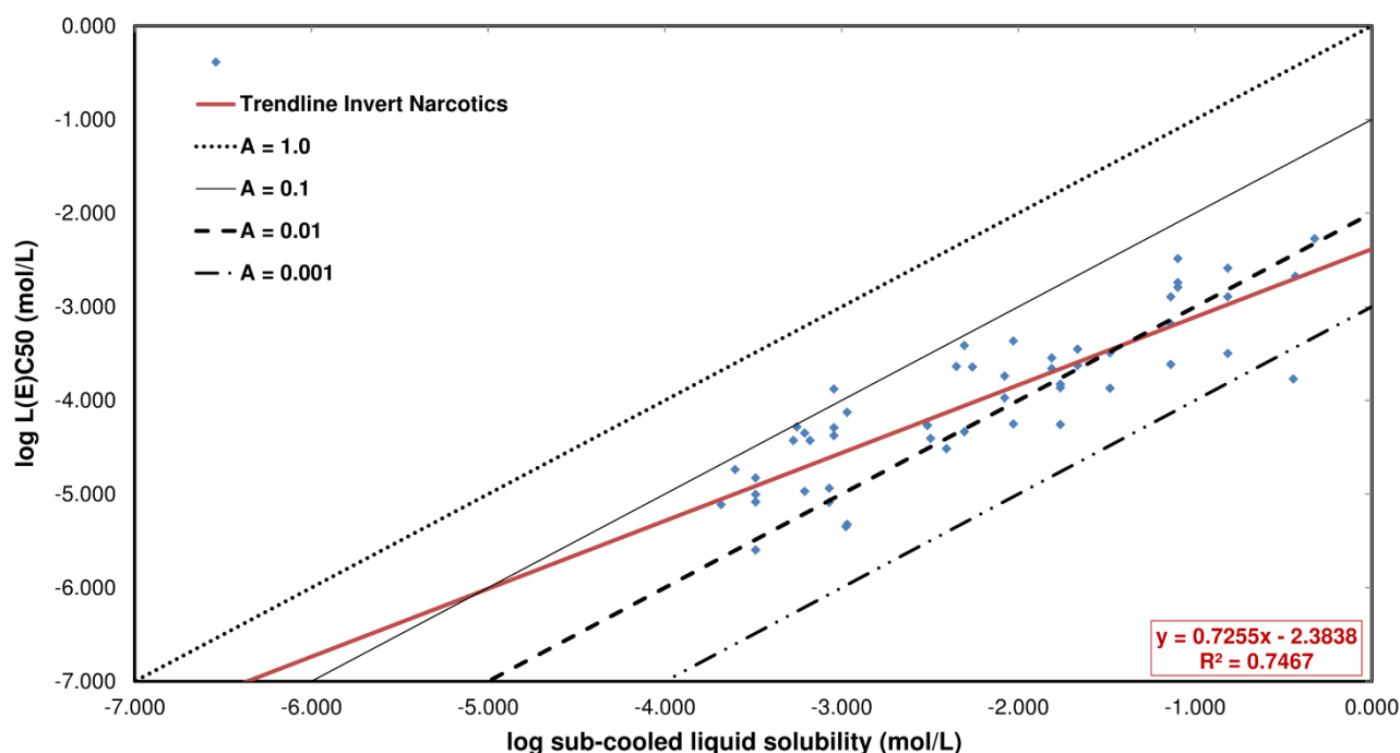
Figure 9: Invert Acute: Narcotics MoA 1
